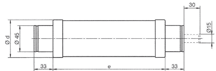
Fig. 2 Dimensions acc. to DIN 43 625 in mm
