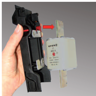
non-contact unlocking of the the Fuse-Link
