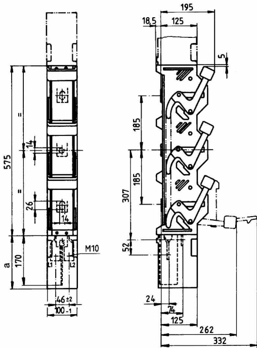
NH Fuse-Switch, vertical design, size 1: 250 A
