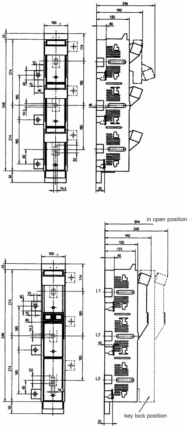
NH Fuse-Switch, vertical design, with sidwise back connection, size 2 - 3: 400 A - 630 A
