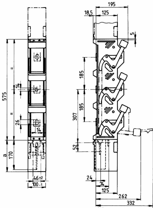
NH Fuse-Switch, vertical design, size 2: 400 A
