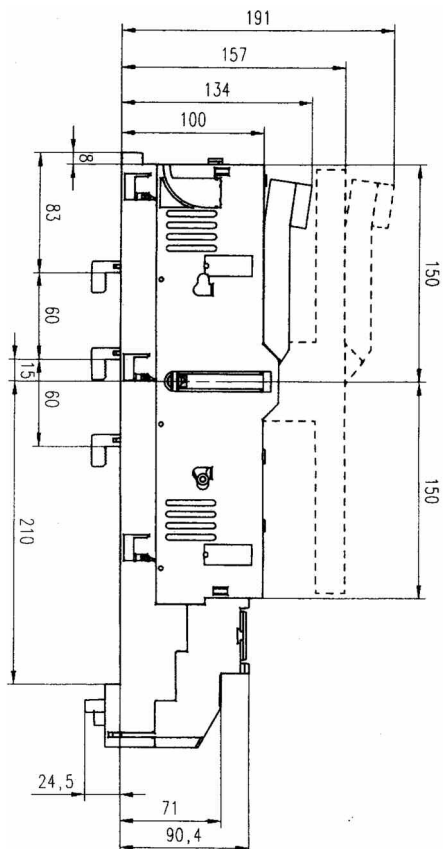
Size 00, Order no.: 38534-1000
