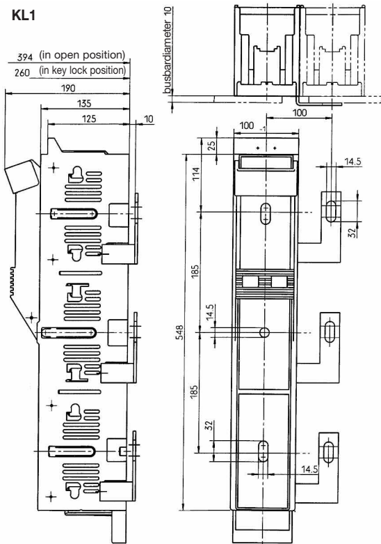
NH Fuse-Switch, size 3, 3-pole switching, with coupling system
